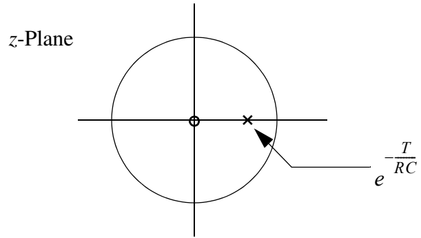
Figure 8: Pole-zero plot of RC low-pass filter following impulse invariant transformation.
