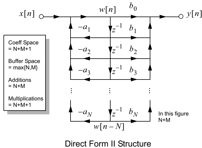
Figure 4: Direct form II structure.
