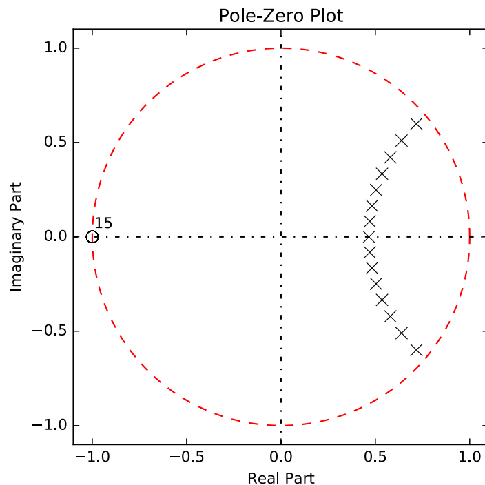
Figure 13: Pole-zero plot of the 15th-order Butterworth design.
