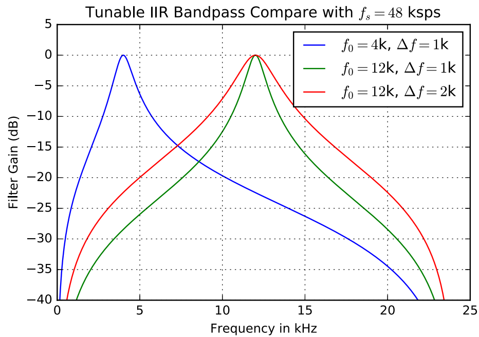
Figure 18: Second-order BPF frequency response magnitude in dB.
