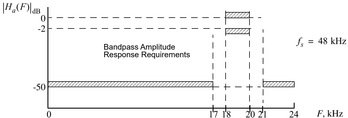
Figure 17: Bandpass filter design requirements.
