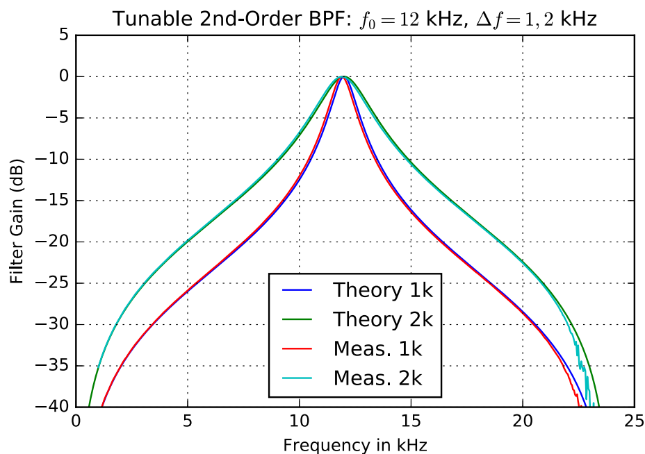
Figure 20: Expected theory versus measured for the tunable bandpass filter app.
