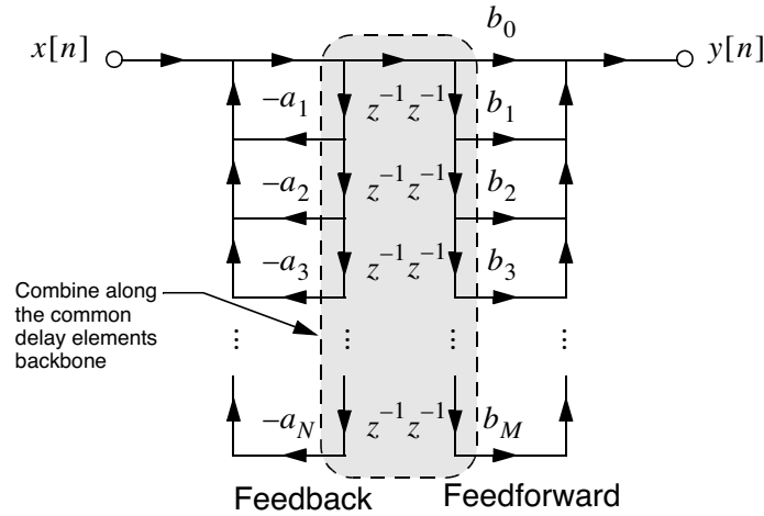
Figure 3: Rearrange the direct form I structure to place the feedback terms first.
