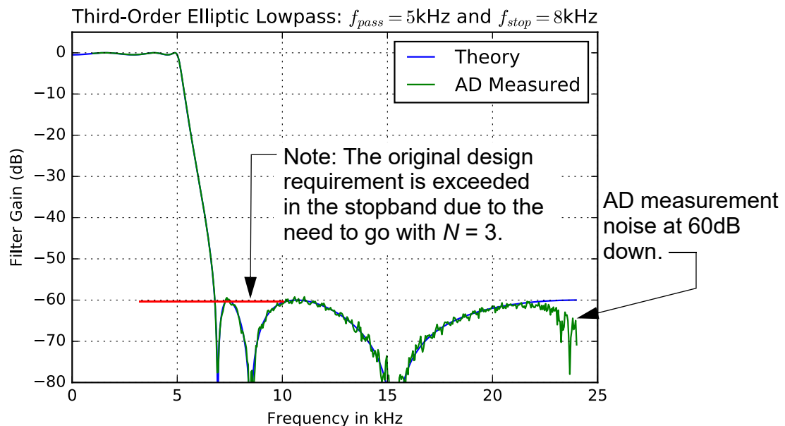
Figure 15: Theory versus measured for the elliptic design example.
