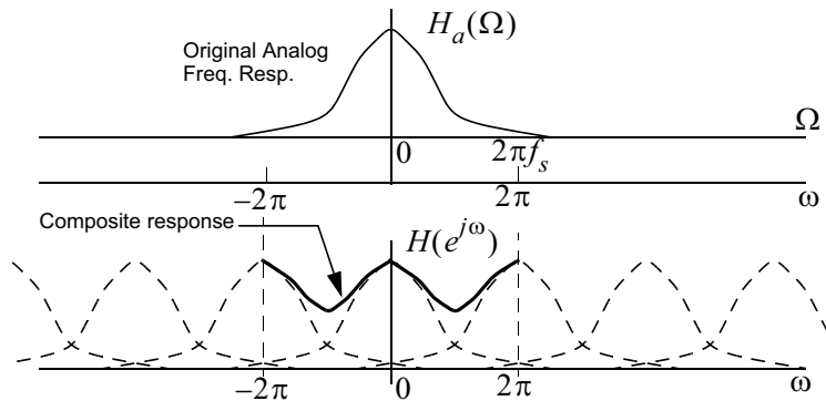
Figure 7: Frequency response of an impulse invariant filter is likely to have some aliasing when compared to the analog prototype.
