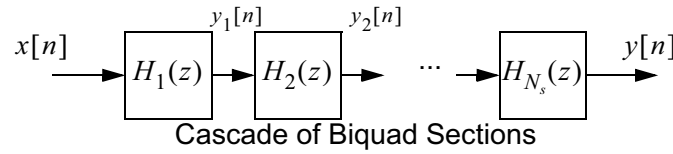
Figure 5: Cascade of biquadratic sections to implement a N > 2 IIR filter.
