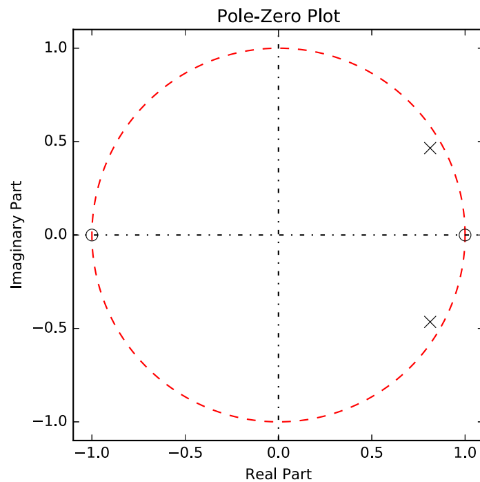
Figure 19: Second-order BPF pole-zero plot for f_0/f_s = 0.125 and \Delta f/f_s = 1/32 .
