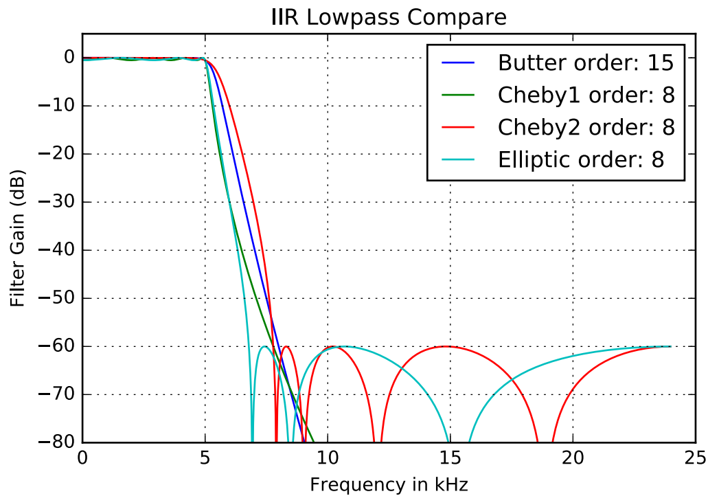
Figure 12: Lowpass comparison plot obtained using freqz_resp_cas_list .
