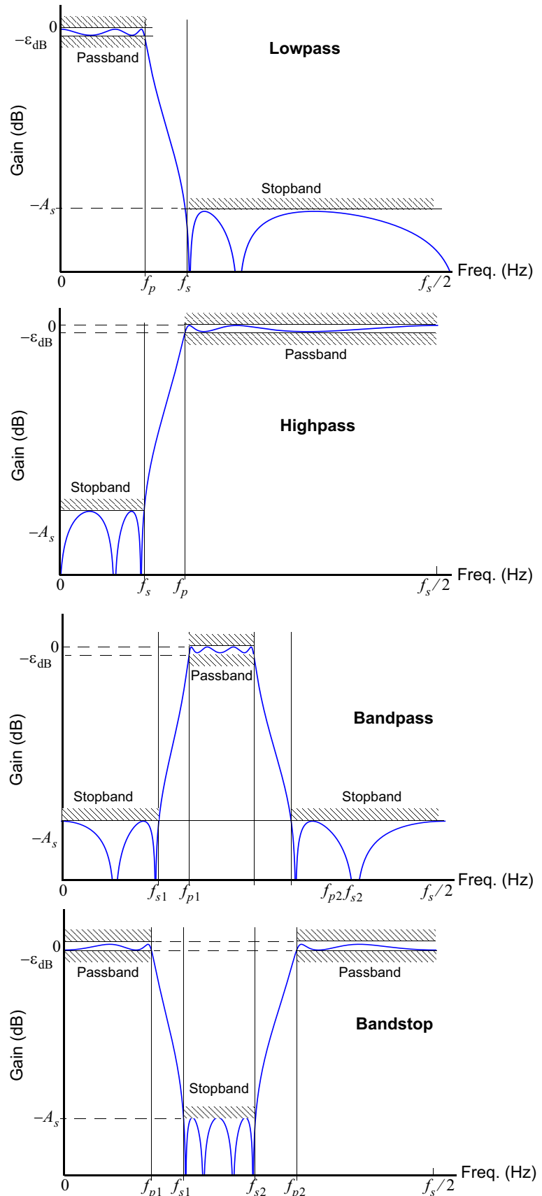
Figure 11: General amplitude response requirements for the lowpass, highpass, bandpass, and bandstop IIR filter types.
