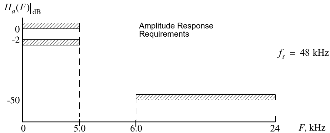
Figure 16: Lowpass filter design requirements.
