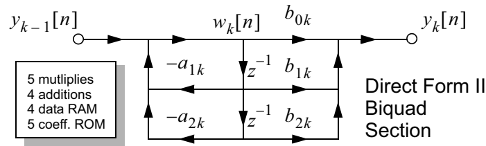
Figure 6: Detailed view of the direct form II biquadratic section.
