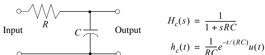
Figure 1: RC lowpass filter.
