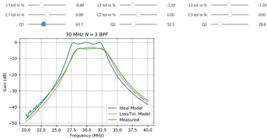
Figure 12: 30 MHz bandpass filter, theory, loss/tolerance model tweaked , and the actual measured response.
