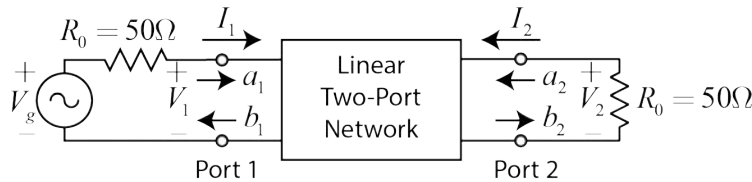
Figure 3: Two-port linear network showing voltage and current relationships along with the normalized incident and reflected wave variables a_i and b_i for i = 1, 2 .
