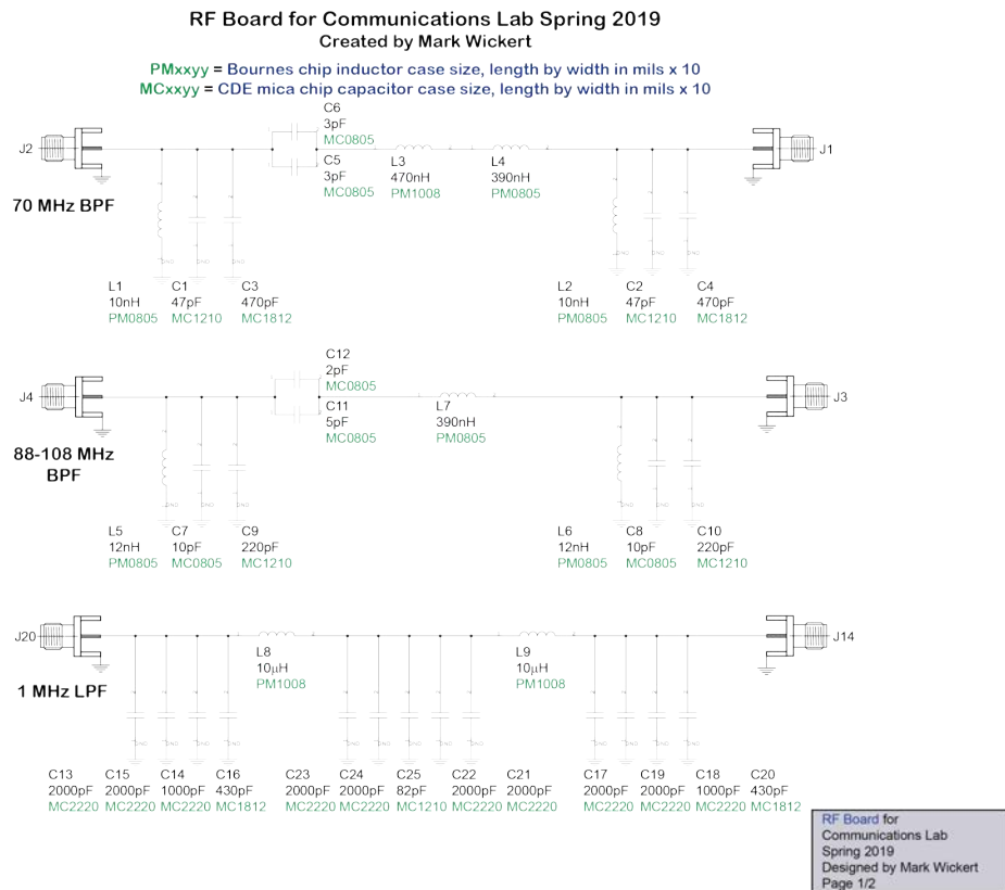
Figure 19: RF board schematic page one showing the passive LC filter designs.
