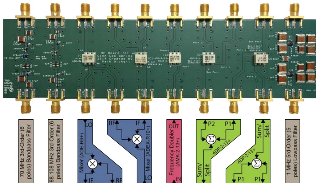
Figure 16: RF board photograph and block diagram of subsystems: 3 filters, 2 mixers, 1 doubler, 2 splitters.
