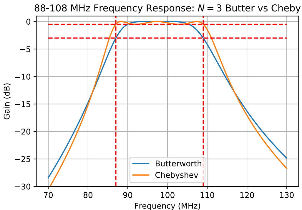
Figure 6: Frequency response magnitude in dB of Butterworth and Chebyshev bandpass filters obtained using a behavioral level model of the analog filter.
