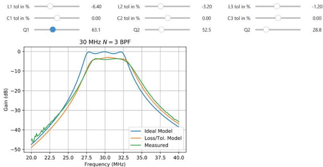
Figure 21: Jupyter interface for studying tolerance and loss in passive LC filters.
