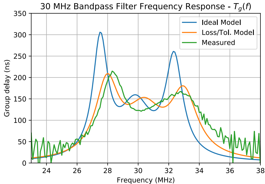
Figure 13: Group delay comparison of theory, L value tweaked with loss model, and measured comparison.
