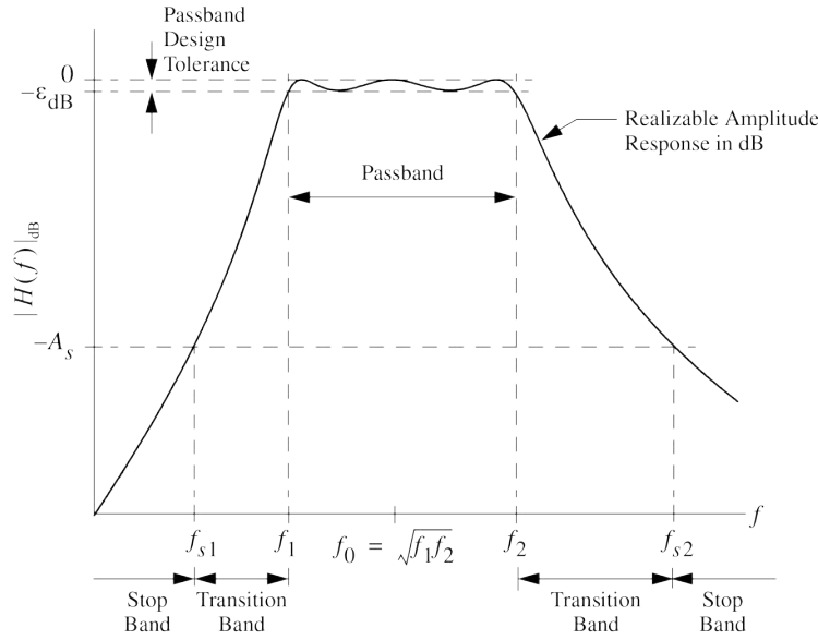
Figure 5: The frequency response of a realizable bandpass filter showing how amplitude response specifications are satisfied by a particular design.
