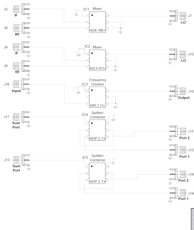
Figure 20: RF board schematic page two showing the Mini Circuits RF components, used in later labs.
