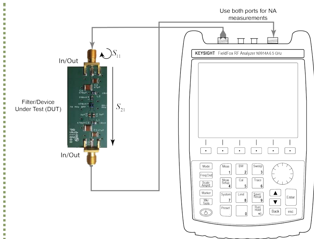
Figure 18: Test setup for measuring the S-parameters of a filter using the N9914A.
