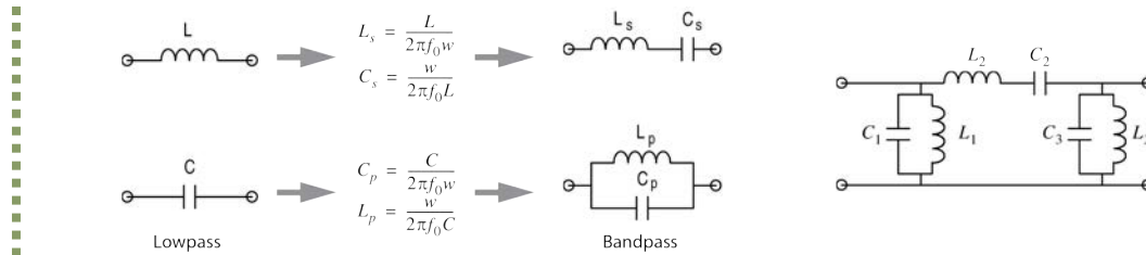
Figure 10: Lowpass to bandpass transformation for the case of a N = 3 bandpass design (6 poles in the bandpass).
