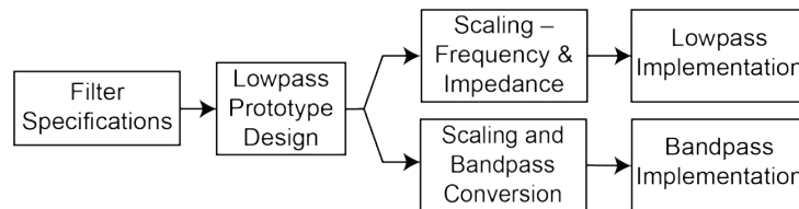
Figure 4: Analog filter design by the insertion loss method.
