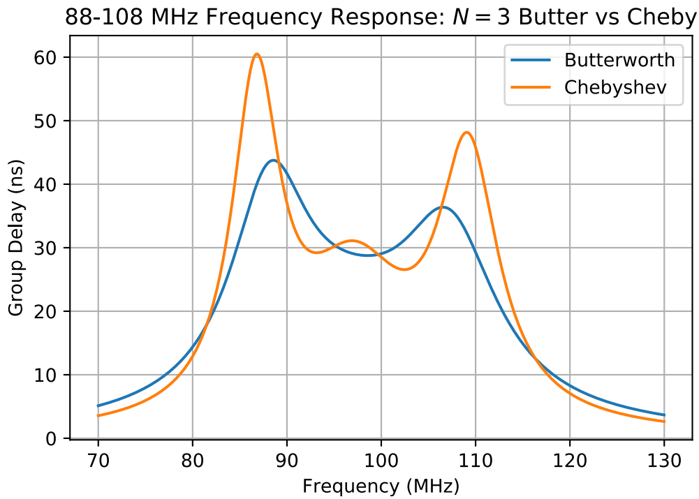
Figure 8: Frequency response group delay of Butterworth and Chebyshev bandpass filters obtained using a behavioral level model of the analog filter.
