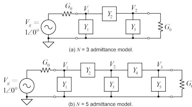
Figure 11: Modeling the N = 3 and N = 5 LC ladder networks using admittances so that component variation and loss due to unloaded Q can be represented.
