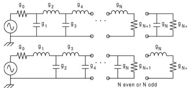
Figure 9: Prototype lowpass filter LC ladder networks, in two equivalent forms, for making both bandpass and lowpass filters.
