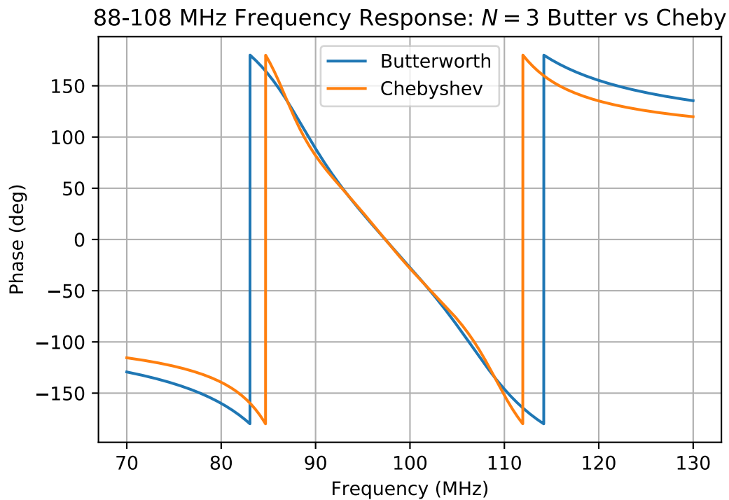
Figure 7: Frequency response phase of Butterworth and Chebyshev bandpass filters obtained using a behavioral level model of the analog filter.
