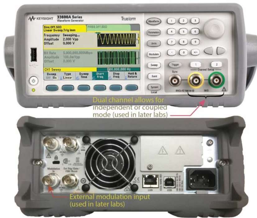
Figure 15: The Keysight 33600A signal generator, front and back.
