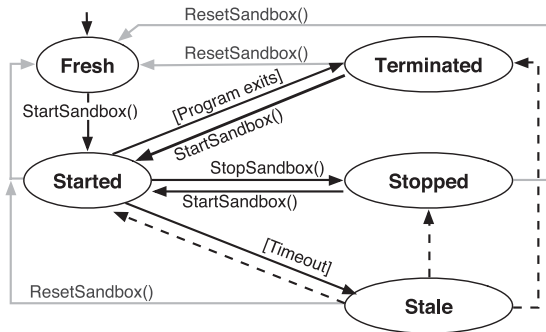
Fig. 2. The sandbox state machine maintained by the resource manager. StartSandbox , StopSandbox , and ResetSandbox are resource manager calls. [Program exits] and [Timeout] are sandbox events. Dashed arrows indicate an implicit event in which the sandbox recovers after a timeout.
